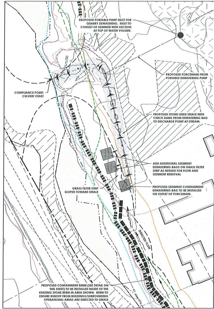
STORMWATER INSET 1" = 30'
